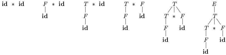
Figure 4.25: A bottom-up parse for \text{id} * \text{id}
