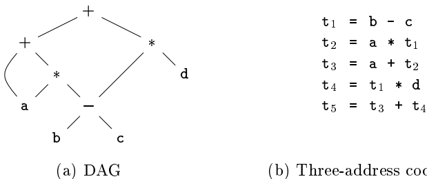
Figure 6.8: A DAG and its corresponding three-address code
