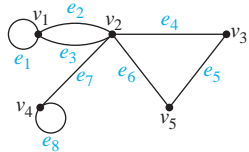
FIGURE 7 A Pseudograph.
