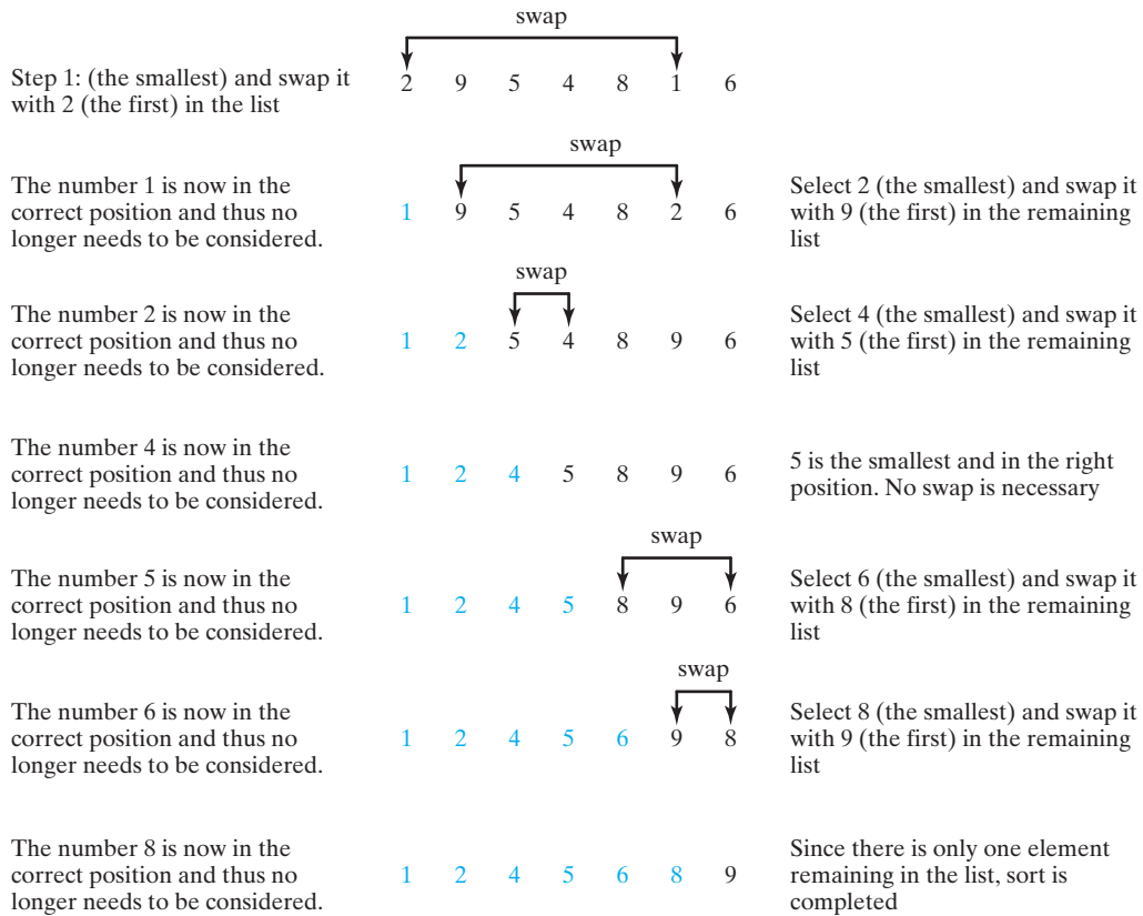
FIGURE 6.11 Selection sort repeatedly selects the smallest number and swaps it with the first number in the list.
