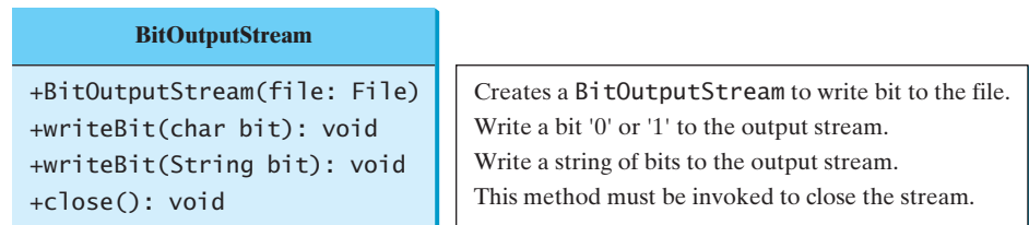
FIGURE 19.20 BitOutputStream outputs a stream of bits to a file.
