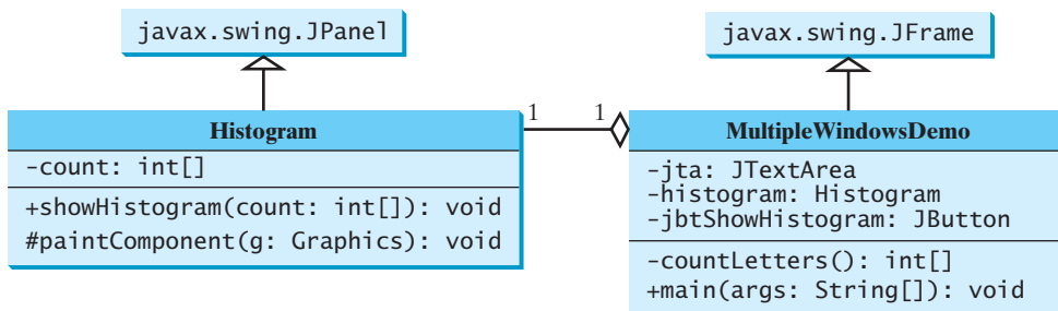
FIGURE 17.32 MultipleWindowsDemo uses Histogram to display a histogram of the occurrences of the letters in a text area in the frame.
