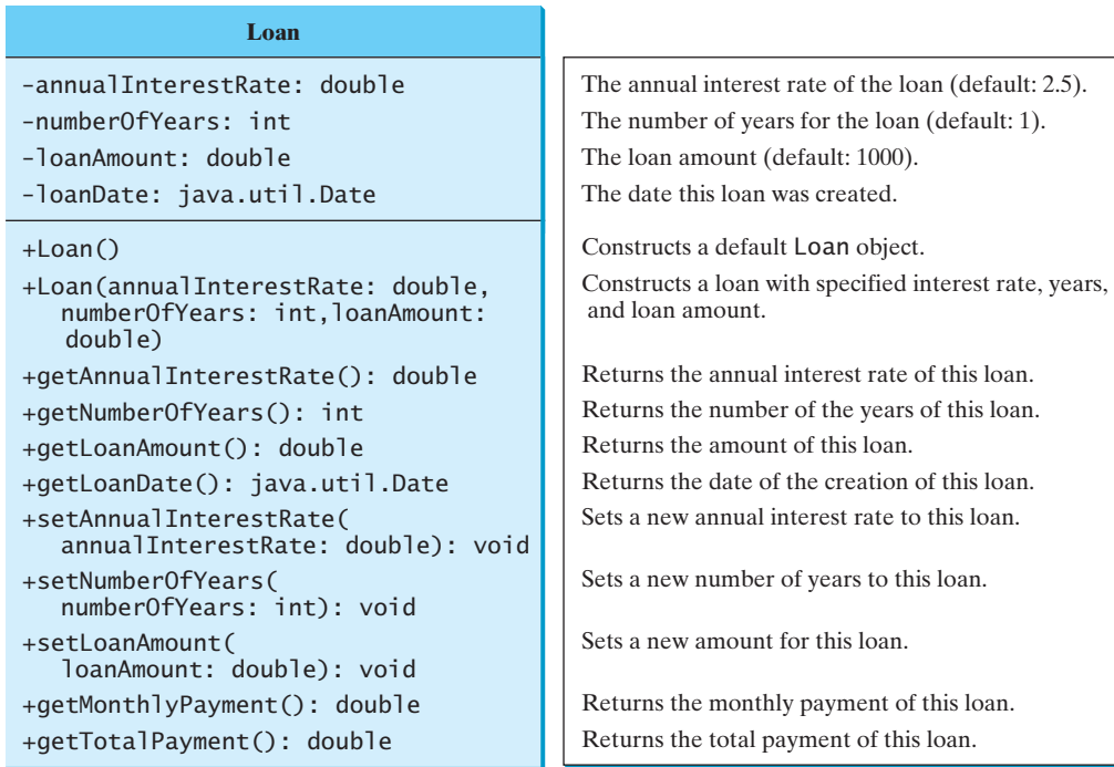
FIGURE 10.4 The Loan class models the properties and behaviors of loans.
