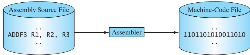
FIGURE 1.3 Assembler translates assembly-language instructions to machine code.
