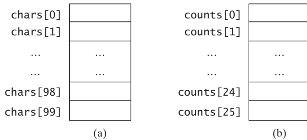
FIGURE 6.7 The chars array stores 100 characters, and the counts array stores 26 counts, each of which counts the occurrences of a letter.
