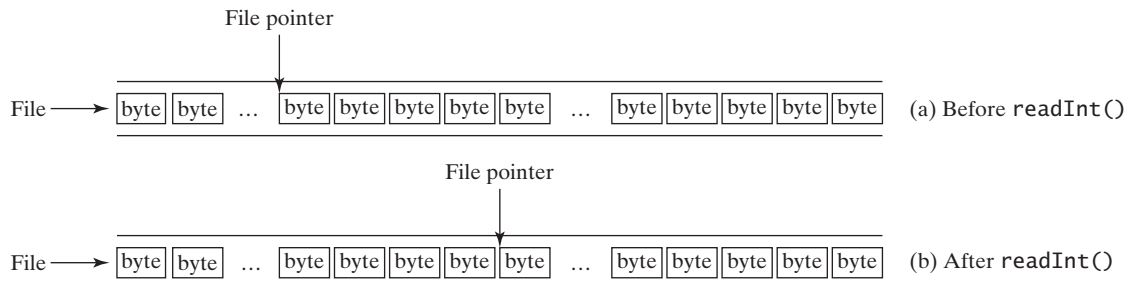
FIGURE 19.17 After an int value is read, the file pointer is moved 4 bytes ahead.
