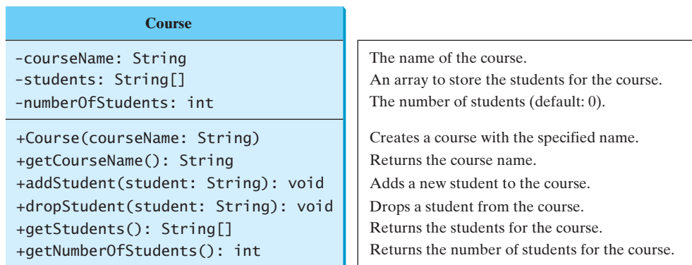
FIGURE 10.9 The Course class models the courses.
