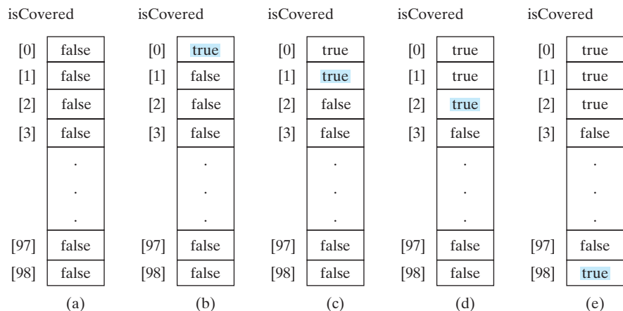
FIGURE 6.2 If number i appears in a Lotto ticket, isCovered[i-1] is set to true.
