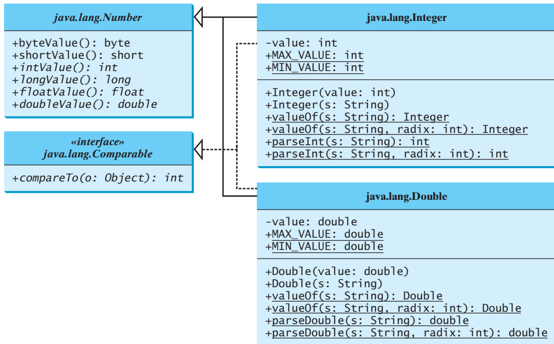
FIGURE 14.9 The wrapper classes provide constructors, constants, and conversion methods for manipulating various data types.
