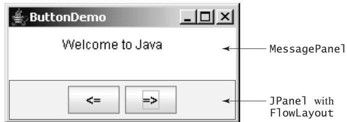
FIGURE 17.9 Clicking the <= and => buttons causes the message on the panel to move to the left and right, respectively.
