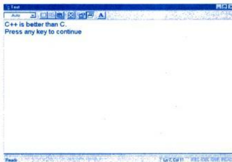
Fig. C.9 ⇔ Output generated
