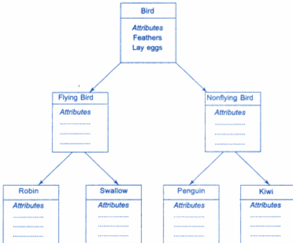
Fig. 1.8 ⇒ Property inheritance
